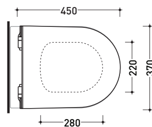
art. 5064 vista zenitale / zenital view
