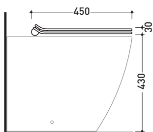
art. LK117 - LK117G - LK117RG vista laterale / lateral view
