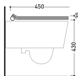
art. 5064 vista laterale / lateral view
